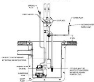
Typical Installation with Submersible Pump and Separate Discharge Pipe
